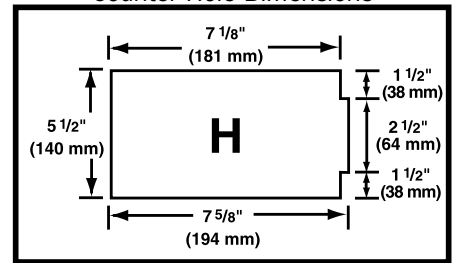
Counter Hole Dimensions
