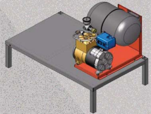
Model 99-2101 Shelf-Mount (for use on 2 or 3 wide BIB top shelf)
