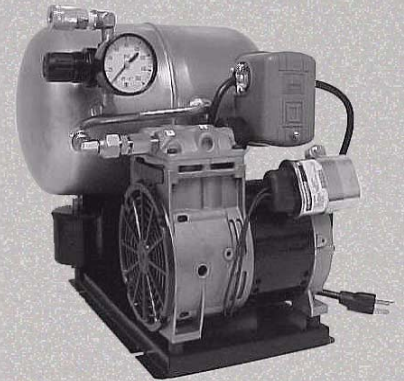
Model 99-2101 Shelf-Mount (for use on 2 or 3 wide BIB top shelf)
