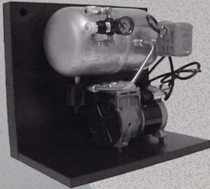
Model 99-2201 Wall-Mount
