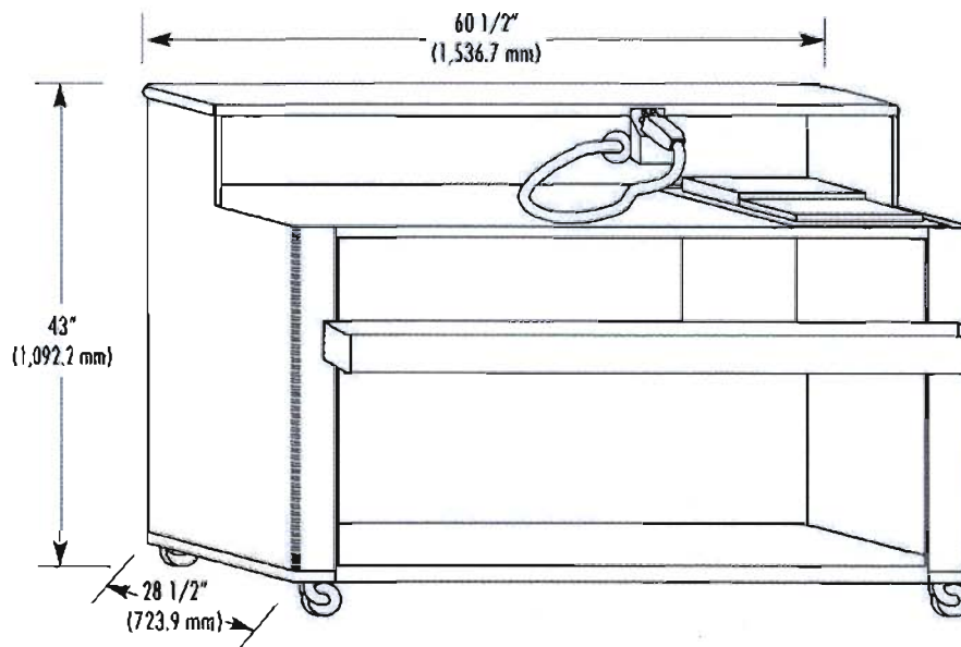
2860R Deluxe Portable Bar
