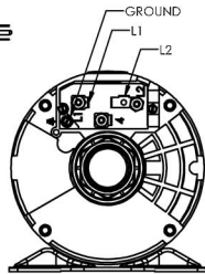
MOTOR WIRE CONNECTION DETAIL
