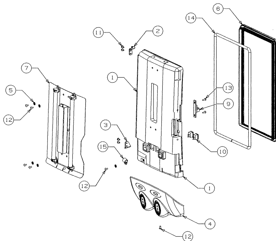
Figure 6. Door Assembly
