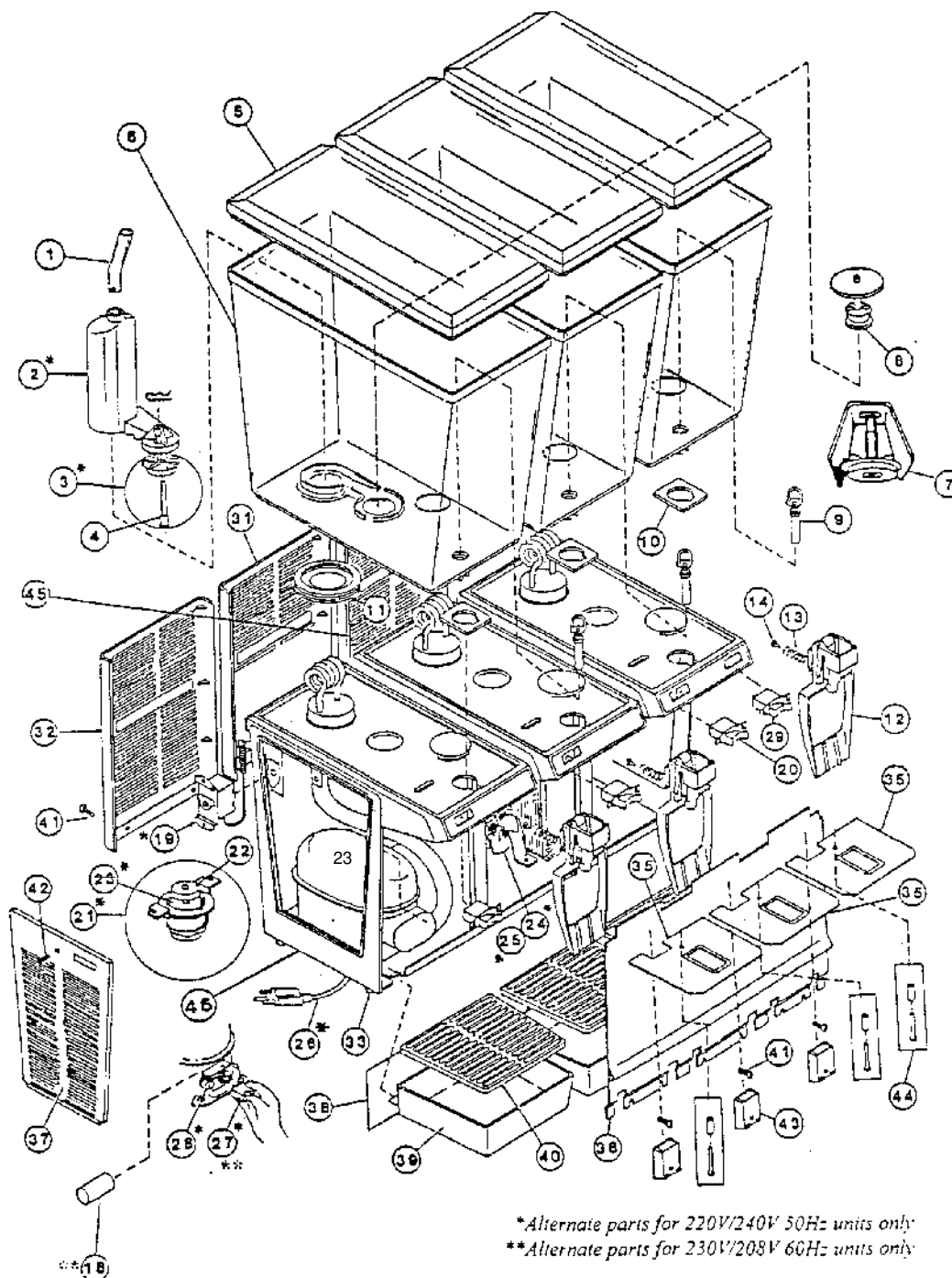
FIGURE 1. GENERAL ASSEMBLY
