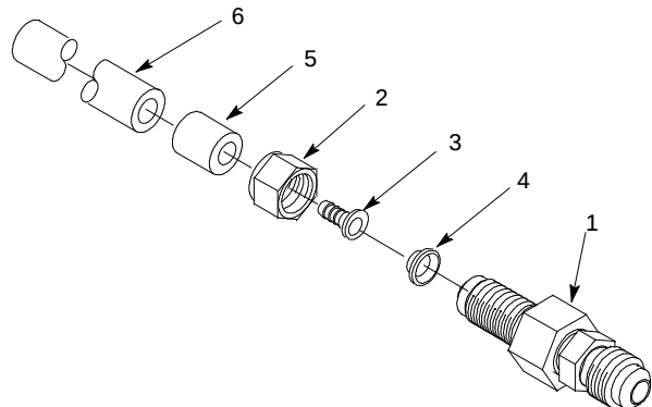
FIGURE 4. TUBE WITH CHECK VALVE ASSEMBLY
