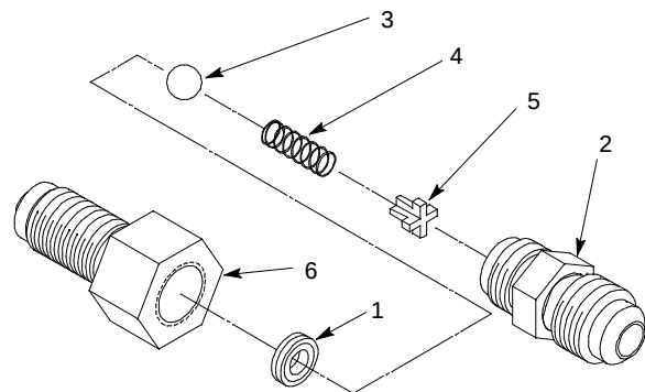
FIGURE 5. CHECK VALVE ASSEMBLY
