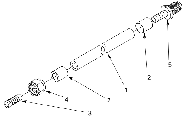
FIGURE 6. TUBE ASSEMBLY
