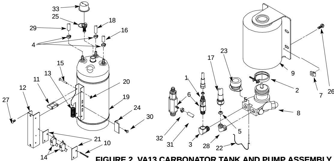
FIGURE 2. VA13 CARBONATOR TANK AND PUMP ASSEMBLY
