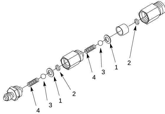
FIGURE 9. LIQUID DUAL CHECK VALVE ASSEMBLY
