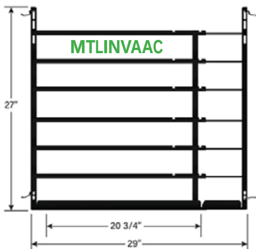
Expandable Add-A-Shelf Top View - Expandable Dimensions
